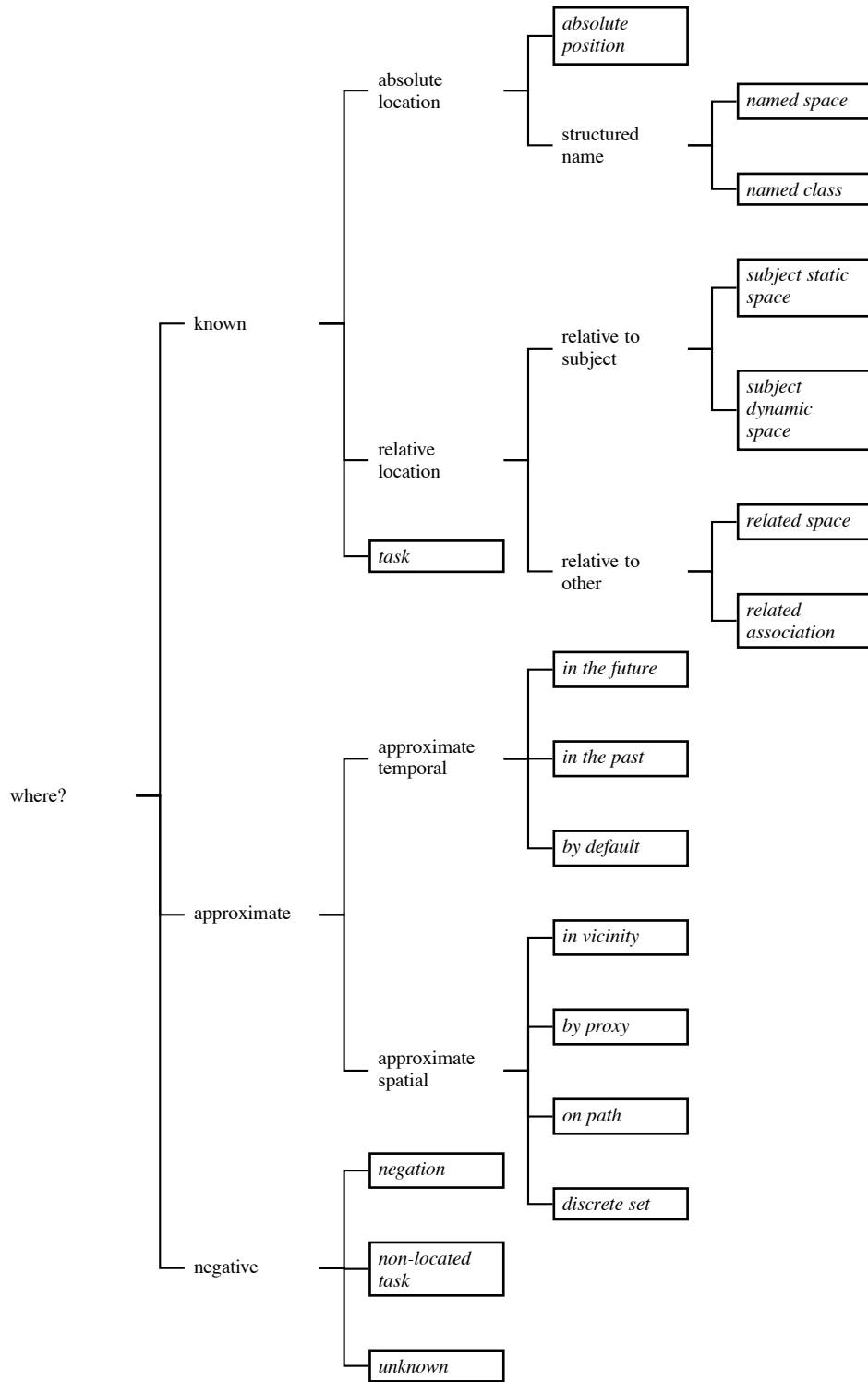
Figure 1. A taxonomy of location in pervasive computing
